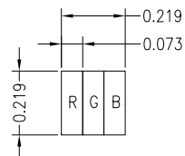
PIXEL DETAIL (SCALE 50:1)
